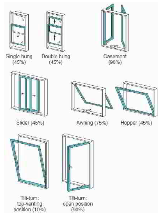
Gambar 4. Ragam Desain Buka-an Sumber: http://inspectapedia.com/BestPractices/Definitions_of_Window_Types.php , diakses 10 November 2015
