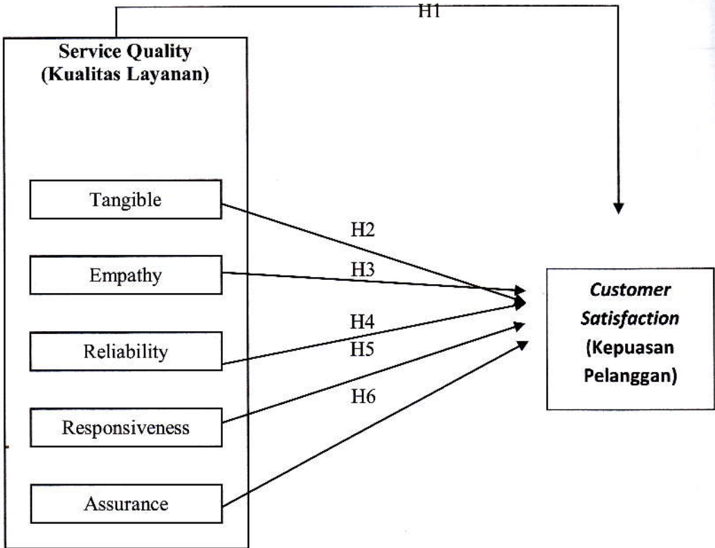
Gambar 1. Model Penelitian
