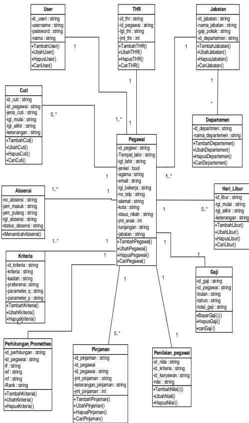
Gambar 1. Class Diagram
