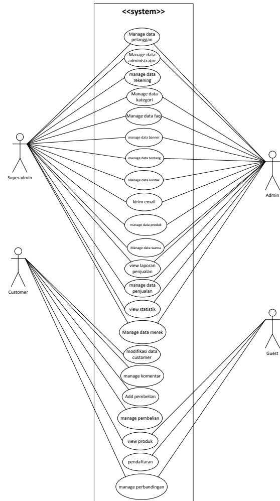
Gambar 1. Use Case Diagram
