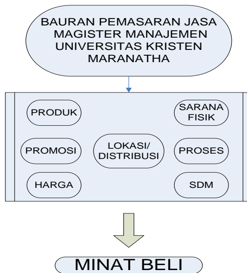
Gambar 2 : Model Penelitian
