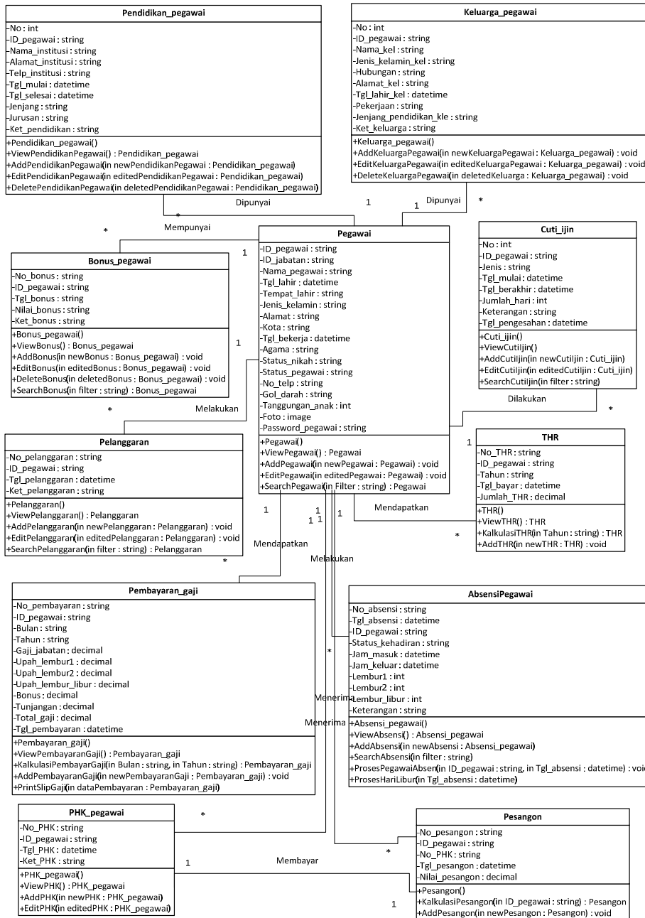
Gambar 3 Class Diagram
